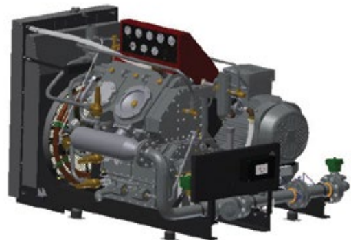
Skid mounted compressor and inlet train with cooling system
